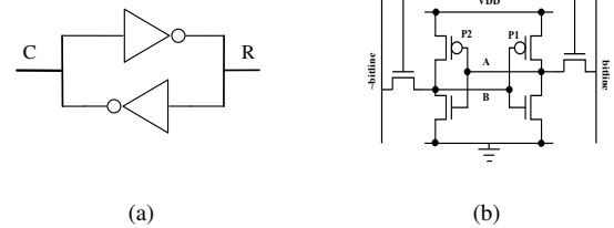
FIGURE 3: Conventional SRAM PUF design by [14]. (a) Gate level. (b) Cell level
