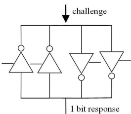
FIGURE 18: 2-stage TSRAM PUF.
